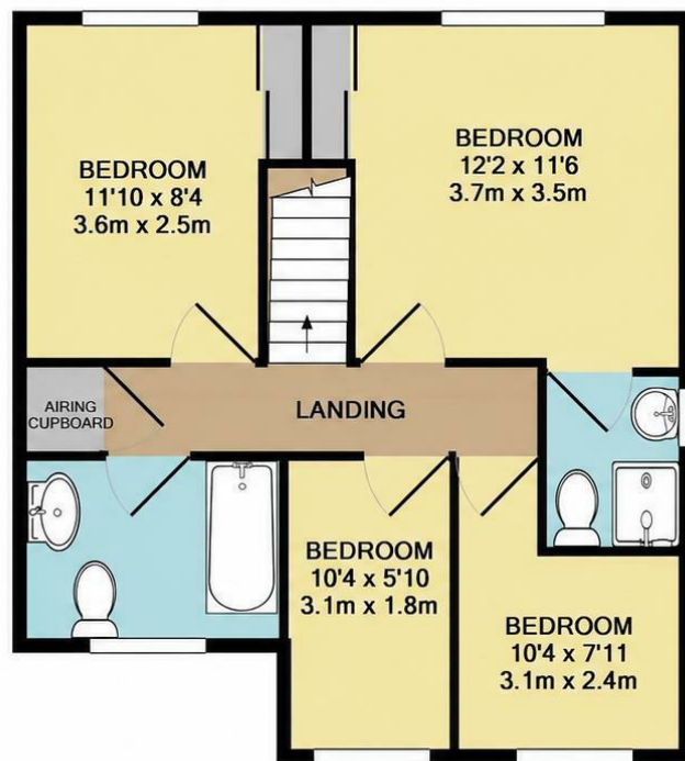
1ST FLOOR APPROX. FLOOR AREA 50.5 SQ.M. (544 SQ.FT.)
