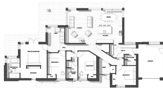
Ground floor 1:100
