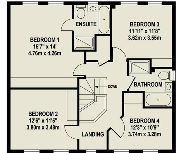
FIRST FLOOR 850 sq.ft. (78.96 sq.m.) approx.
