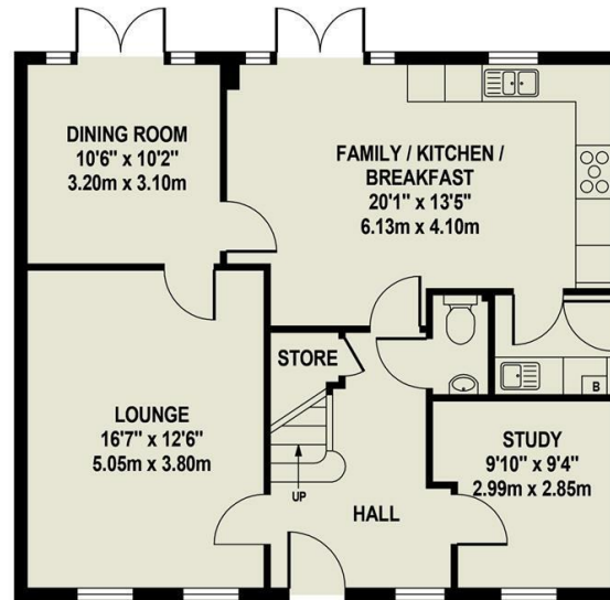
GROUND FLOOR 850 sq.ft. (78.96 sq.m.) approx.
