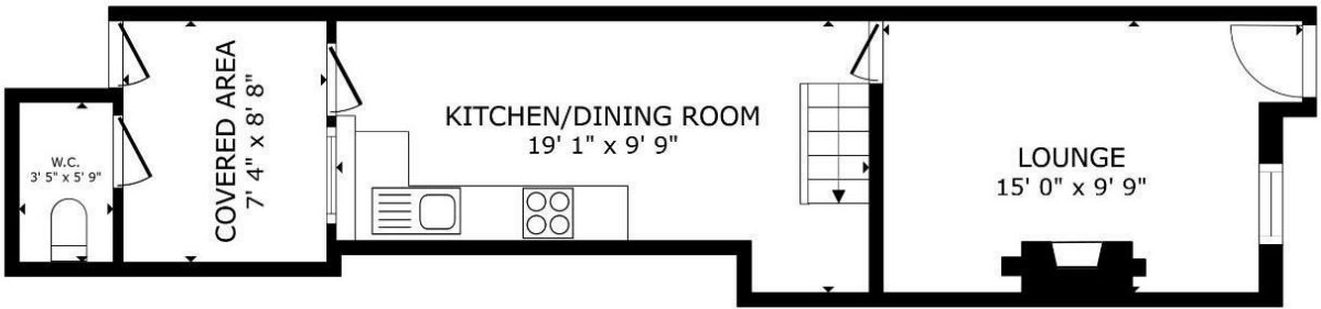
FLOOR 1
