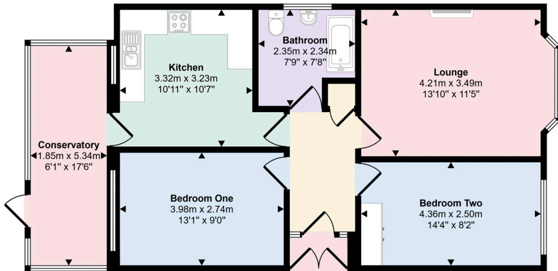
Floorplan
