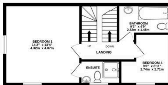
1ST FLOOR 415 sq.ft. (38.5 sq.m.) approx.
