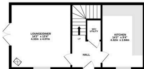
GROUND FLOOR 415 sq.ft. (38.5 sq.m.) approx.
