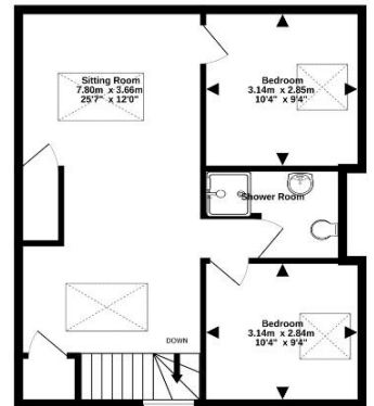
2nd Floor 52.4 sq.m. (564 sq.ft.) approx.
