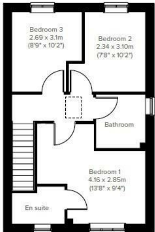
1ST FLOOR
