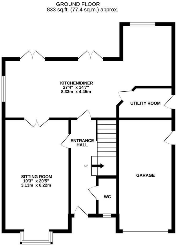
TOTAL FLOOR AREA : 1470 sq.ft. (136.6 sq.m.) approx. Whilst every attempt has been made to ensure the accuracy of the floorplan contained here, measurements of doors, windows, rooms and any other items are approximate and no responsibility is taken for any error, omission or mis-statement. This plan is for illustrative purposes only and should be used as such by any prospective purchaser. The services, systems and appliances shown have not been tested and no guarantee as to their operability or efficiency can be given. Made with Metropix ©2026
