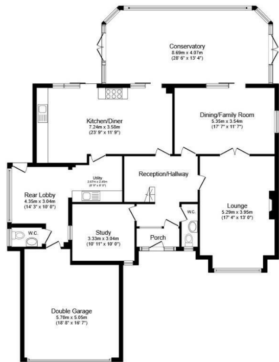
Ground Floor Floor area 183.3 sq.m. (1,973 sq.ft.)
