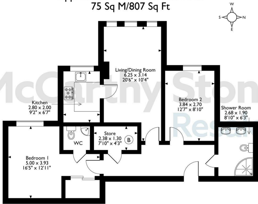
Second Floor The position & size of doors, windows, appliances and other features are approximate only. © ehouse. Unauthorised reproduction prohibited. Drawing ref. dig/8659294/DST.
