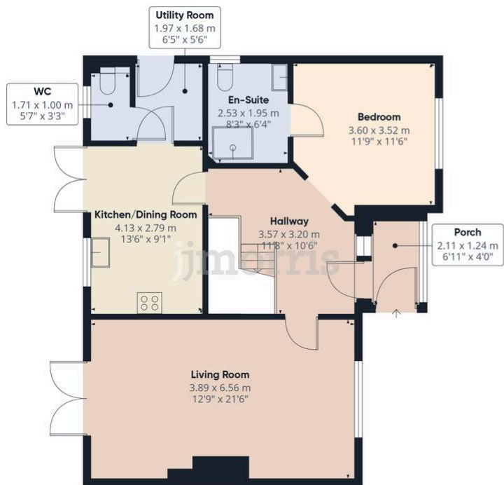
Floor 0 Building 1
