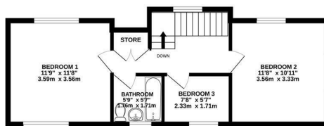
1ST FLOOR 430 sq.ft. (39.9 sq.m.) approx.
