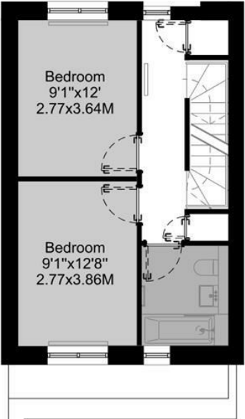
First Floor 405 SQ FT
