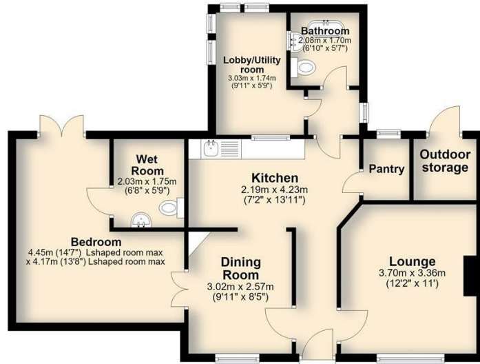
Ground Floor Approx. 68.6 sq. metres (737.9 sq. feet)
