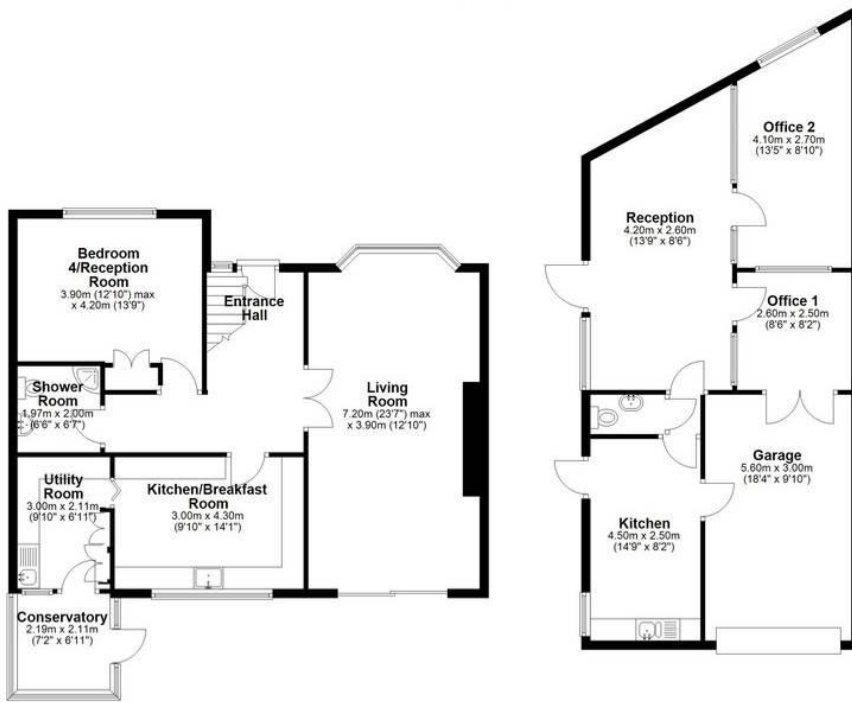
Ground Floor Approx. 158.0 sq. metres (1700.3 sq. feet)
