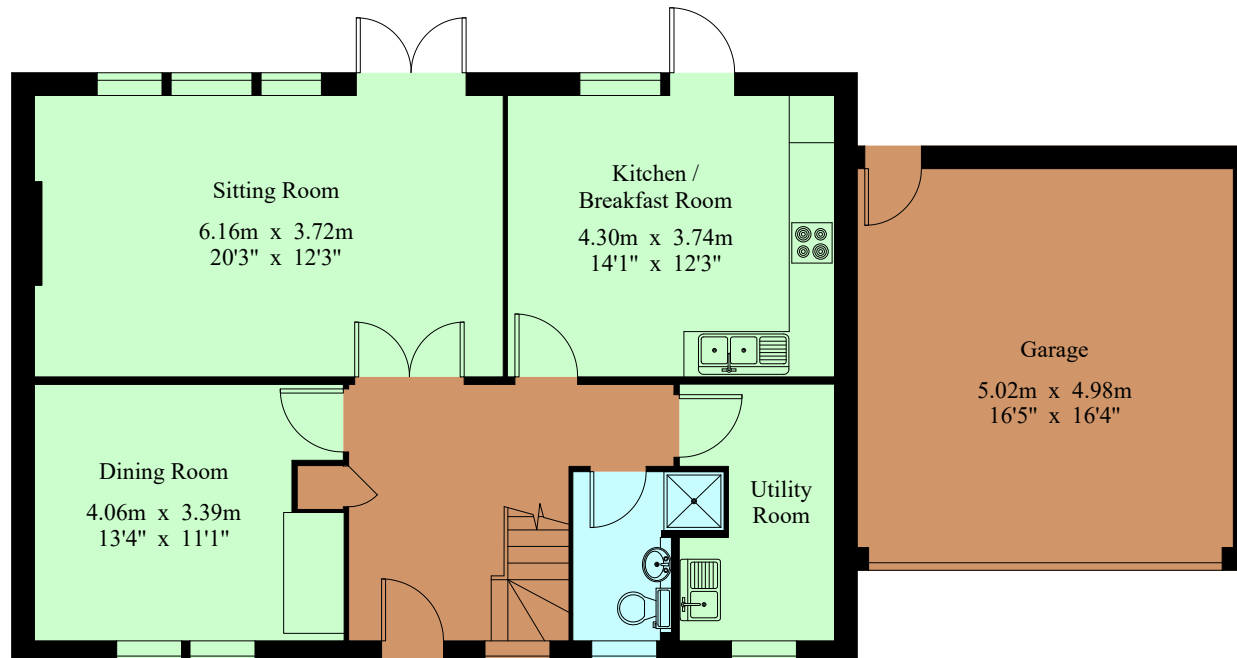
Ground Floor
