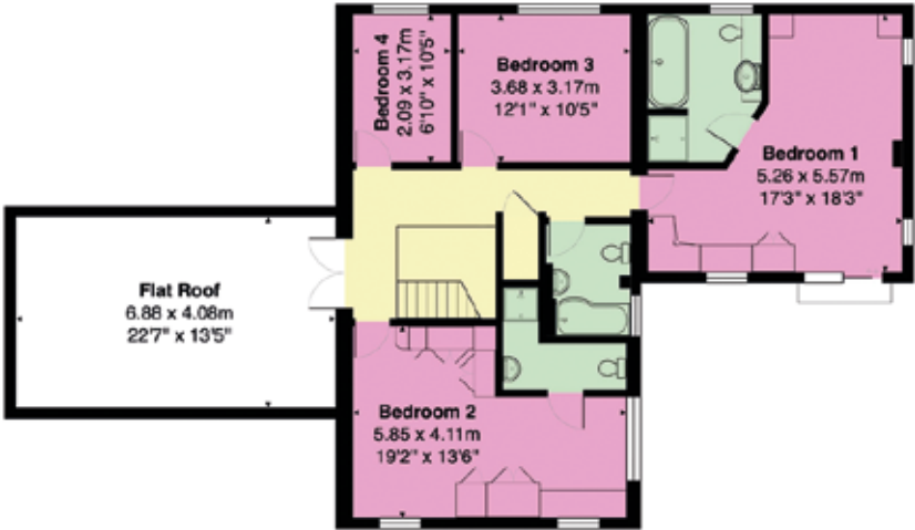
House First Floor
