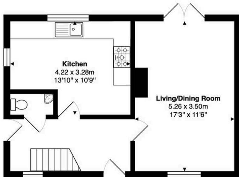
Ground Floor Area: 41.9 m 2 ... 451 ft 2
