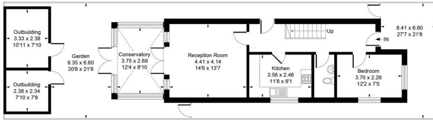
Ground Floor
