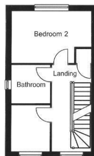
First Floor Plan (not to scale)
