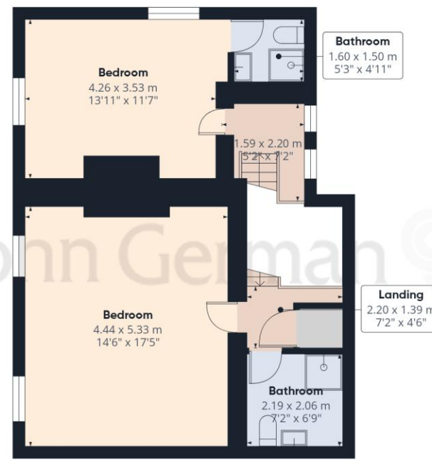
Floor 1 Building 1
