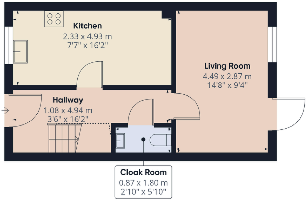
Floor 0
