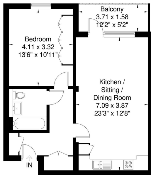
Second Floor
