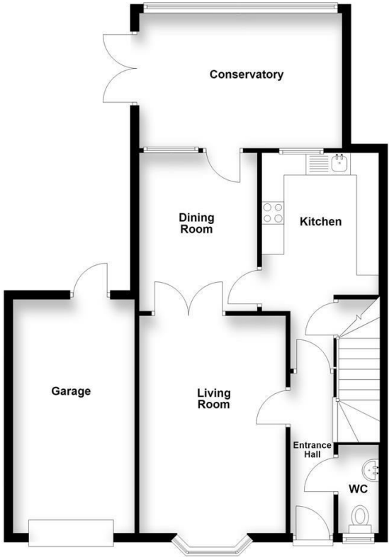
Ground Floor Approx. 75.5 sq. metres (812.9 sq. feet)
