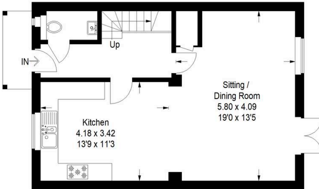
Ground Floor
