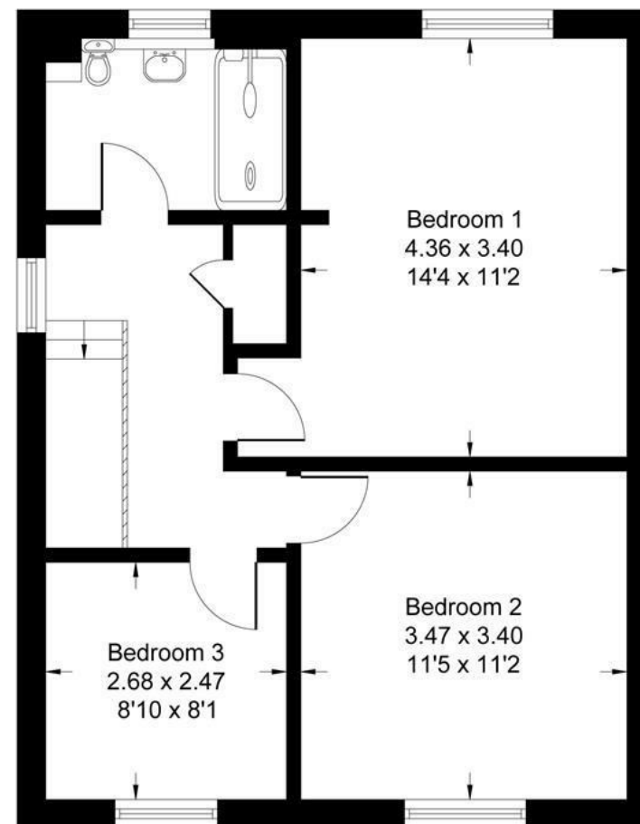
First Floor
