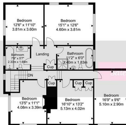
First Floor Approximate Floor Area 1155.39 SQ.FT. (107.34 SQ.M.)
