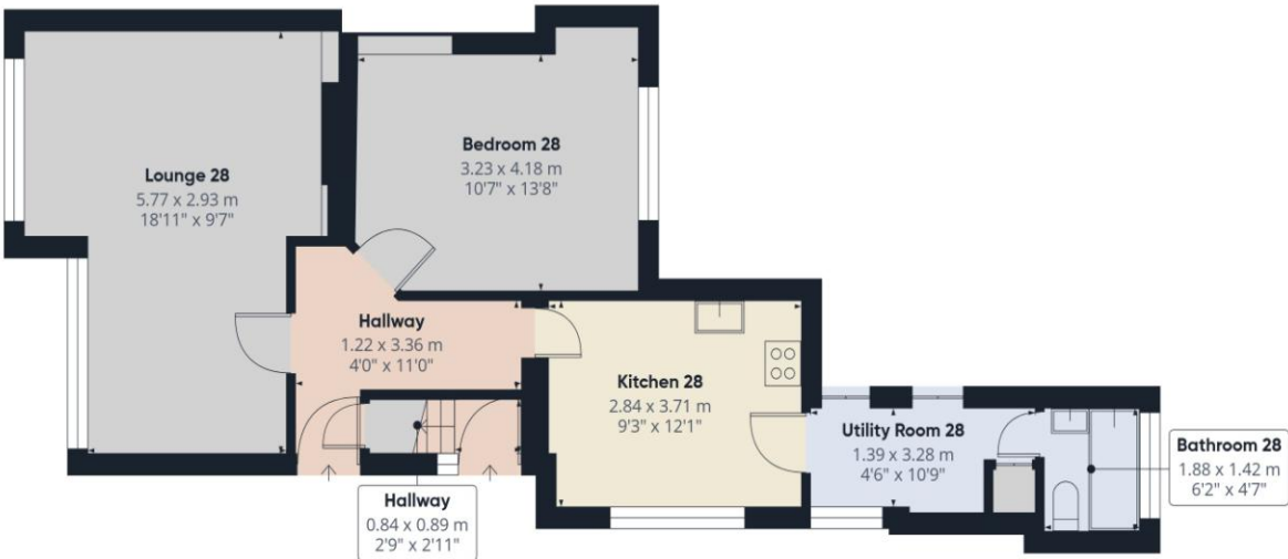
Floor 0
