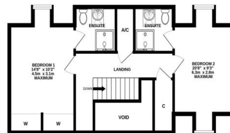
1ST FLOOR 551 sq.ft. (51.2 sq.m.) approx.
