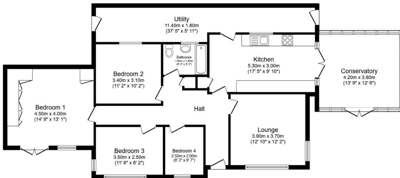
Floor Plan Floor area 129.3 sq.m. (1,392 sq.ft.)
