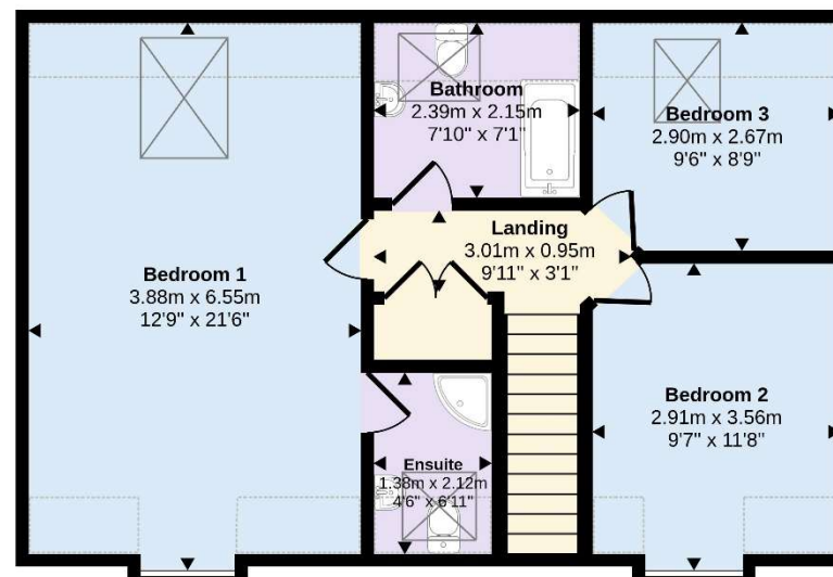
First Floor Approx 60 sq m / 646 sq ft
