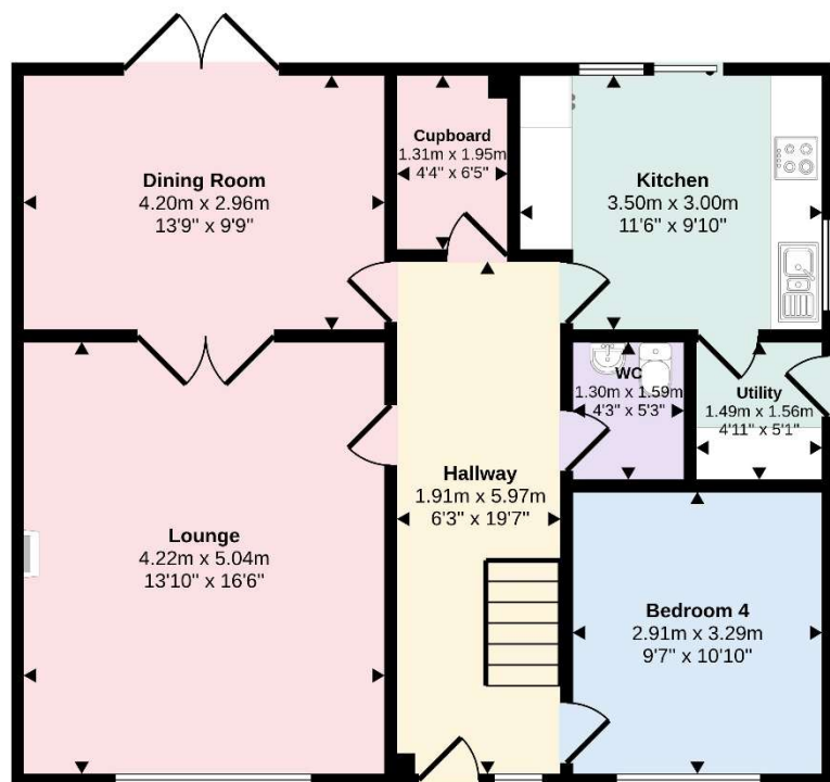
Ground Floor Approx 76 sq m / 818 sq ft
