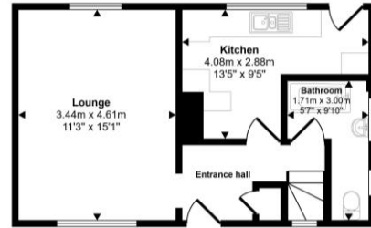
Ground Floor Approx 35 sq m / 382 sq ft
