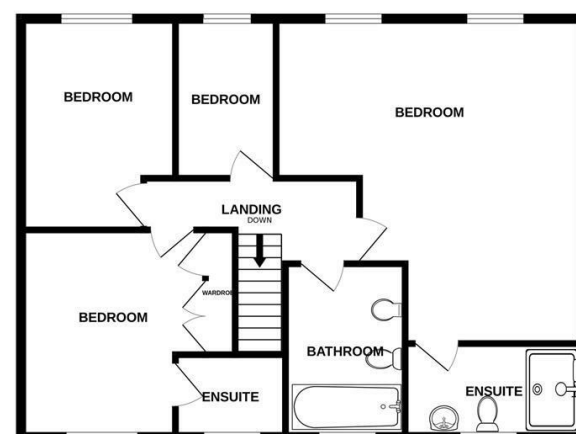
1ST FLOOR 807 sq.ft. (75.0 sq.m.) approx.
