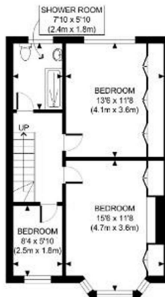
SECOND FLOOR GROSS INTERNAL FLOOR AREA 401 SQ FT
