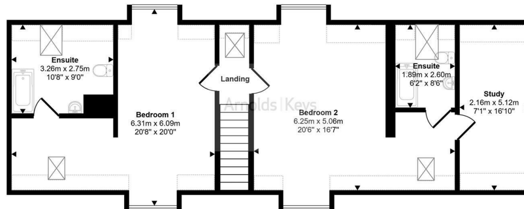
First Floor Approx 86 sq m / 921 sq ft
