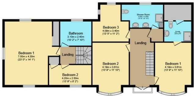
First Floor Floor area 134.7 sq.m. (1,450 sq.ft.)
