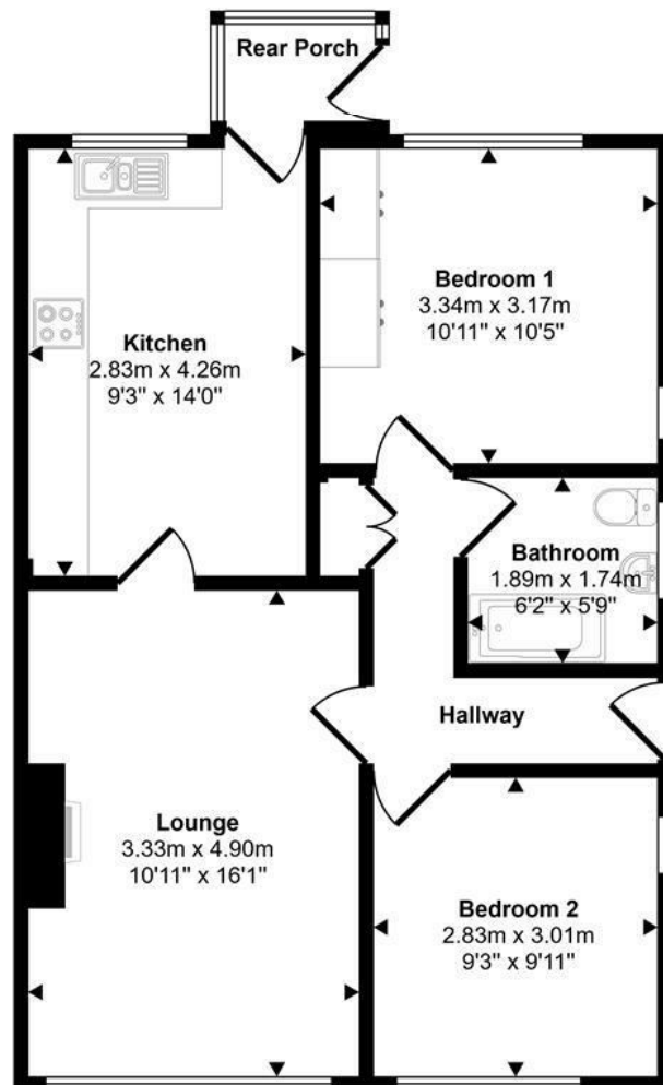
Floorplan
