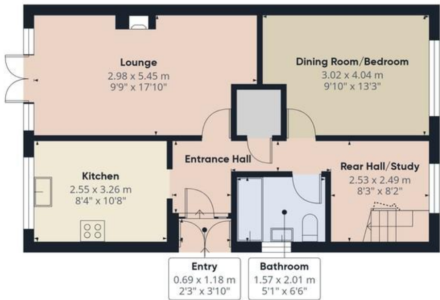
Floor 0
