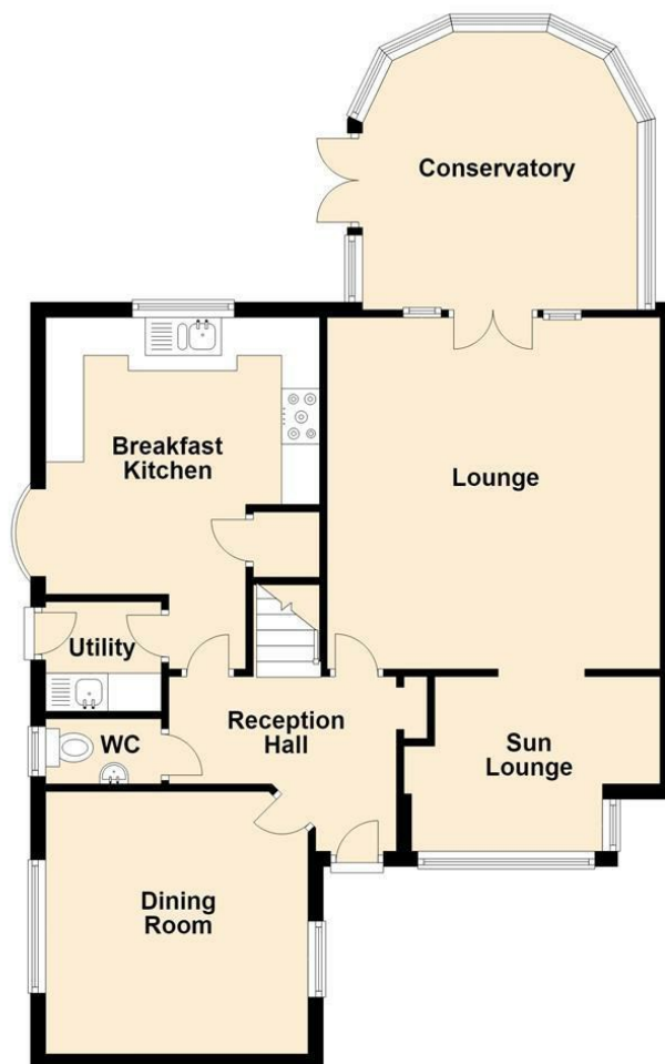
Ground Floor Approx. 78.1 sq. metres (840.2 sq. feet)
