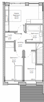
First Floor - Plot 2 1:50
