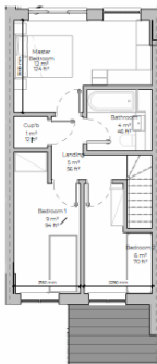
First Floor - Plot 3 1:50
