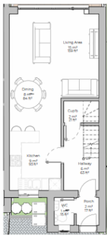
Ground Level - Plot 1 1:50
