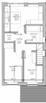
First Floor - Plot 1 1:50
