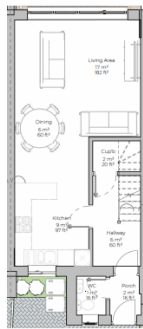
Ground Level - Plot 2 1:50
