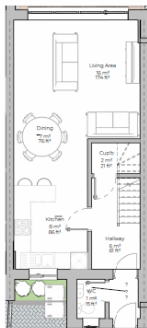
Ground Level - Plot 3 1:50
