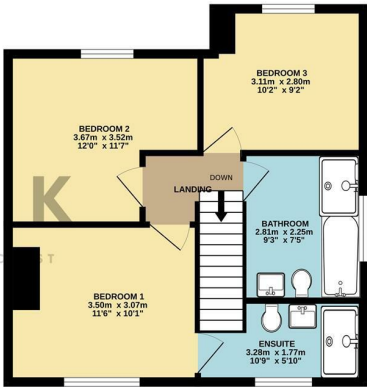
1ST FLOOR 44.0 sq.m. (474 sq.ft.) approx.
