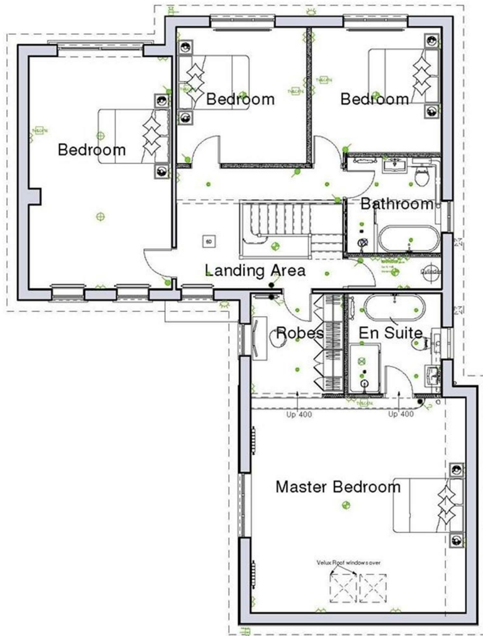
'HEDGEROWS' FIRST FLOOR PLAN
