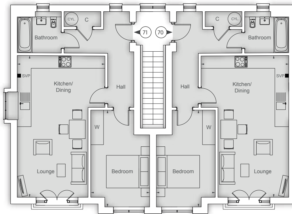
First Floor (plots 70 & 71) 567 sqft 52.7 sqm
