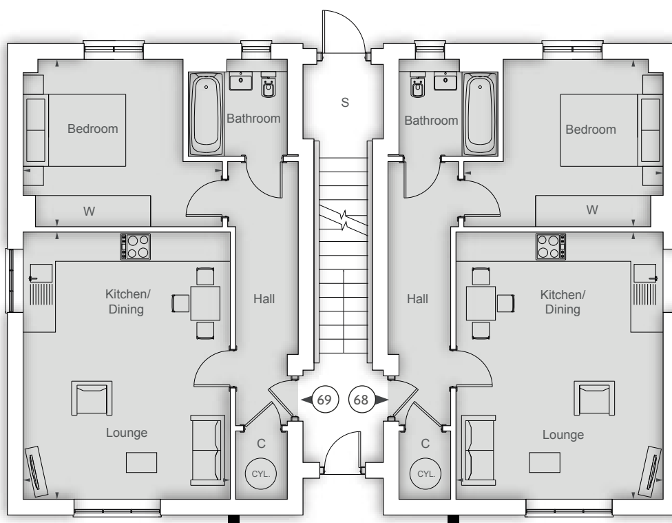
Ground Floor (plots 68 & 69) 524 sqft 48.7 sqm
