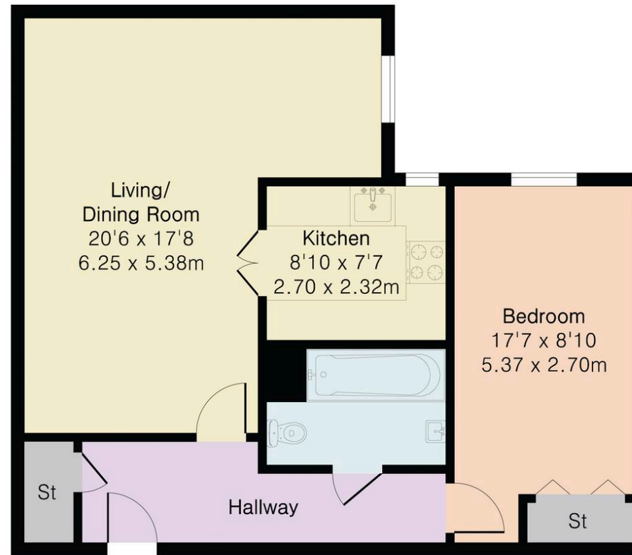
Third Floor
