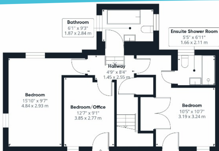
Floor 0
