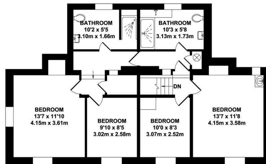
FIRST FLOOR APPROX. FLOOR AREA 815 SQ.FT. (75.72 SQ.M.)
