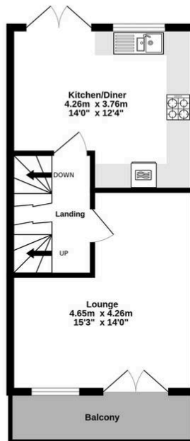
1st Floor 35.8 sq.m. (386 sq.ft.) approx.
