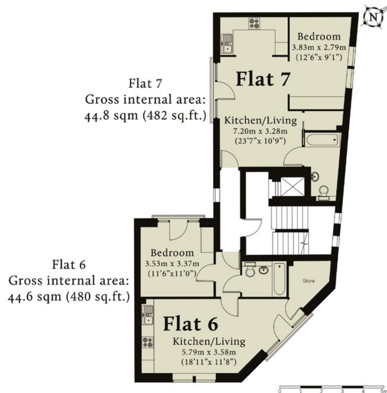
Leeward House: Third Floor
