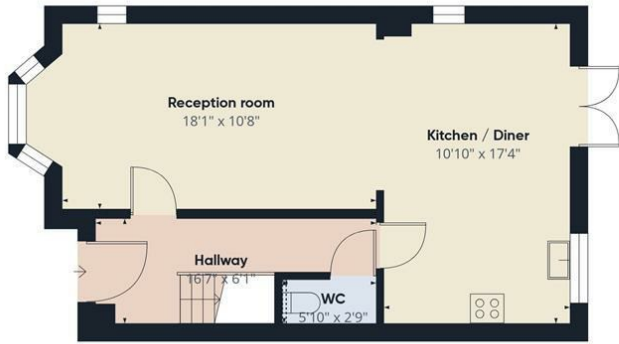
Floor 0 Building 1
